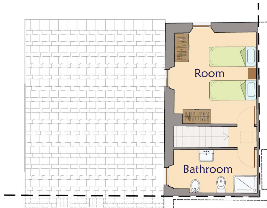
First floor
